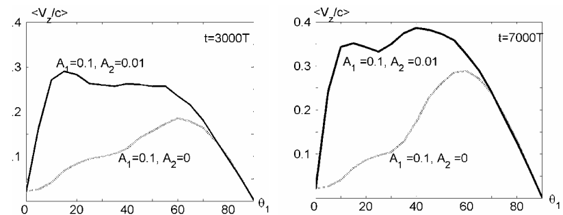
Fig.3 For low density runs n_e \approx 0.6 \times 10^{19} m^{-3} , averaged electron velocity versus the propagation angle of the primary wave \theta_1 (in degrees) at the normalized times: t=3000 (left picture), t=7000 (right picture) for two wave scheme (solid line), and one wave (dotted line)
