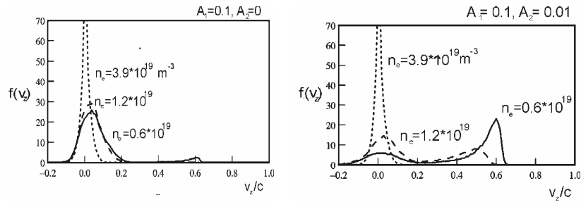
Fig.4. Probability Distribution of the parallel velocity for \theta_1 = 15^\circ
