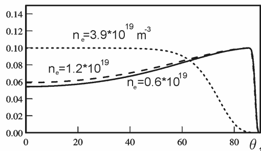
Fig.2 Averaged parallel flux I^* (in arbitrary units) of the particles in the RL as a function of the angle of the primary wave, \theta_1 (in two-wave plane Configuration – Fig.1) for different electron densities. We see a clear maximum of the particle flux at non-zero propagation angle of the primary wave as expected due to asymmetry of the resonance layer (RL) in velocity space and pseudo-stochastization of the particle population by the secondary wave.
