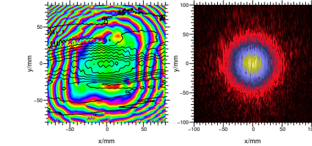
Figure 2: Input distribution with corresponding phase corrector (left) and target distribution (right).
