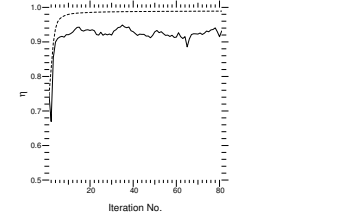
Figure 4: Convergence of the classical (dashed) and modified (solid) KS-Algorithm.
